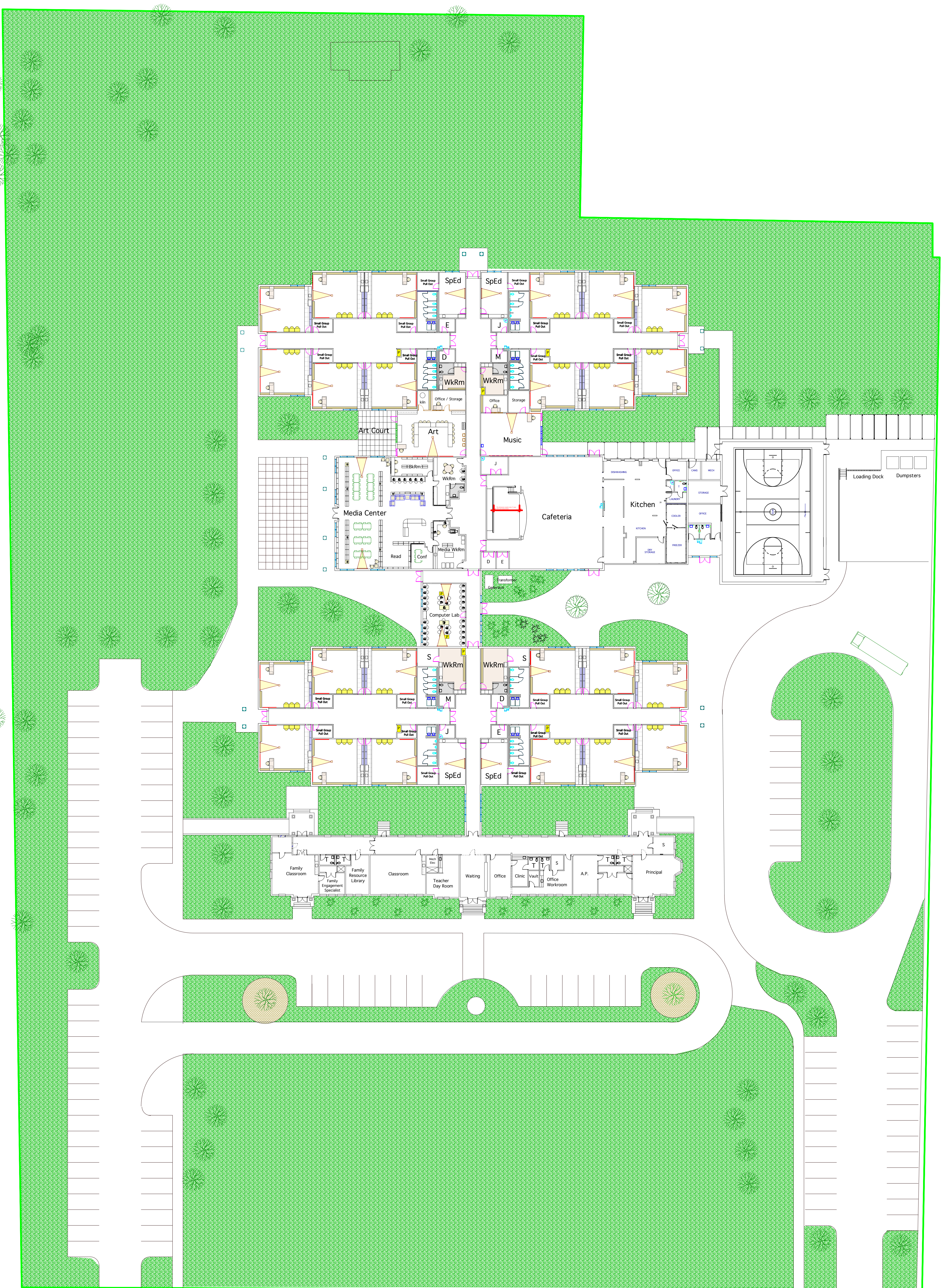
Chase Street Elementary School - April 25, 2006 - Final Draft Plan
